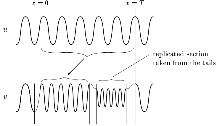
Figure 6: In the case H > 0 the original function u is compressed; a near-optimal section is taken from the tails and replicated to fill the gap.
