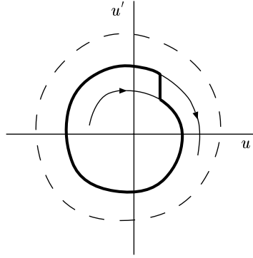
Figure 5: In the half-plane \{u' > 0\} the solution curve moves to the right. Therefore the closed curve forms a barrier that the solution curve can not pass. The limit state (dashed line) is the limit of such closed curves.
