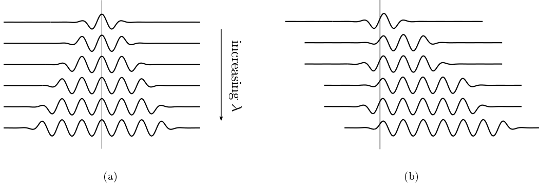
Figure 3: Solutions of (2.1) for different values of \lambda , for the nonlinearity F(u) = u^2/2 - u^4/4 + 0.3 u^6/6 . The vertical lines indicate the different choices of translations: in (a) the solutions are aligned on their maximum, and in (b) on a smallness condition to the left of the line.
