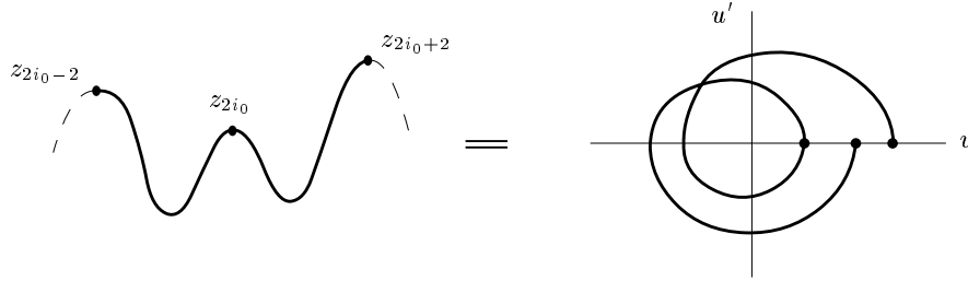
Figure 4: The ordering of the maxima implies the existence of an intersection in the u, u' -plane
