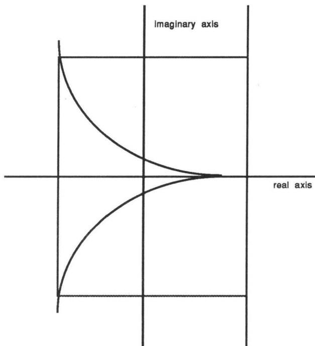
FIGURE 7.1. The contour \Gamma_{\omega_l}(\gamma, \gamma_l) .
