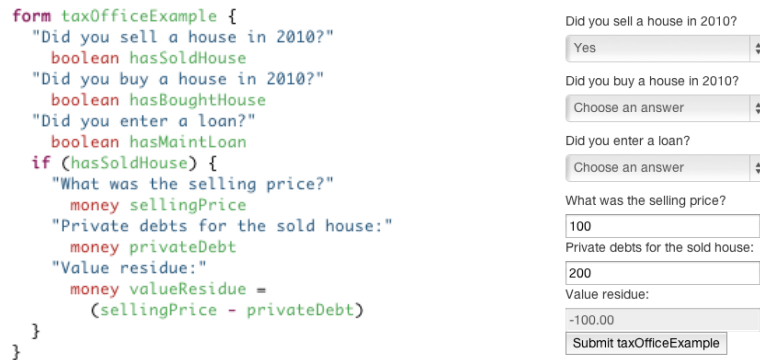
Figure 2: An example of a textual QL model (left) and its default rendering (right).
