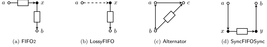
Figure 1: Example connectors.
