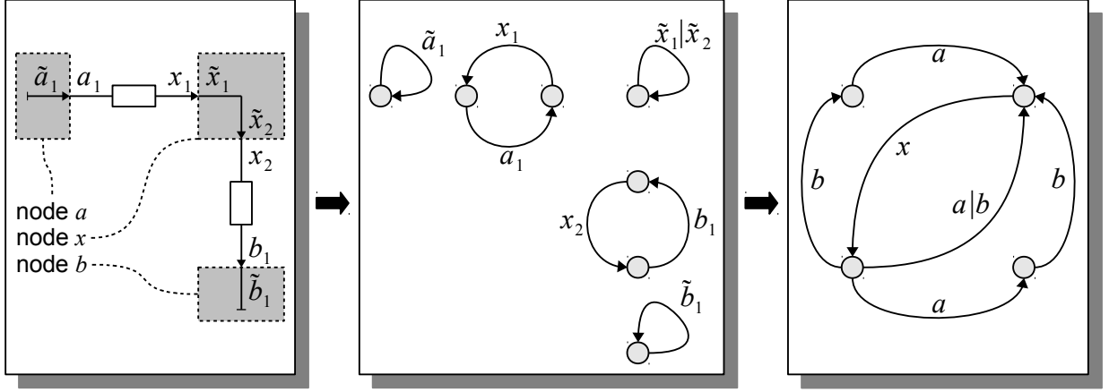
Figure 8: Labeled transition system(s) of the proces(ses) modeling the connector in Figure 1a. On the left is a graphical representation of the decomposition of that connector into channels and nodes with labeled ends. In the middle are the labeled transition systems of the processes modeling those channels and nodes (without data for simplicity). On the right is the labeled transition system of the parallel composition of those processes (after applying communication and blocking).
