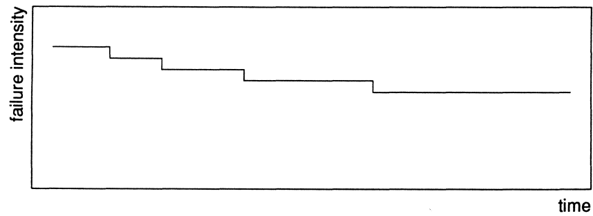
(b) Goel-Okumoto
