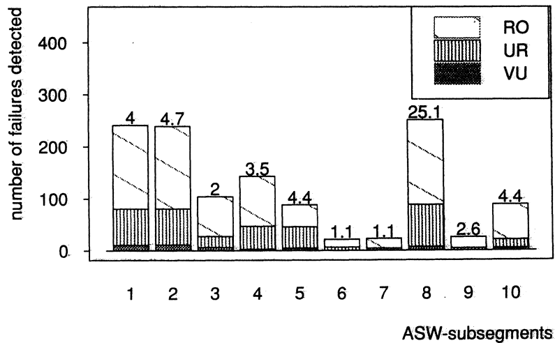
Figure 8.1 ASW-failures since project start (a) Evolution in time (b) Distribution over the ASW-subsegments.
