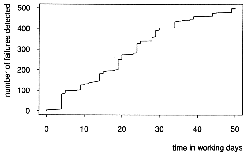
(b) ASW-failures during alpha-test
