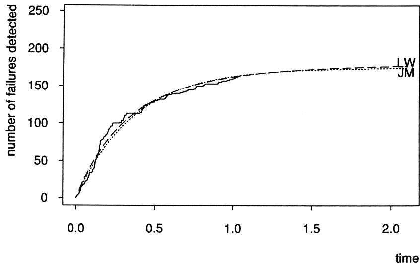
Figure A.1 Real data set (Mellor & Littlewood).
