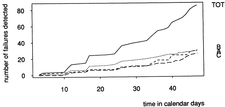
Figure 8.10 Number of faults detected against calendar time.
