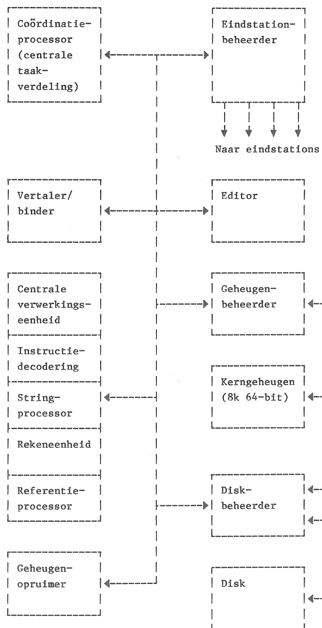
Fig. 1 - SYMBOL blokdiagram
