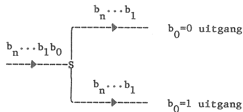
Fig. 10. Selector.
