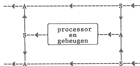
Fig. 12. Communicatie in Barton/Clark cel.
