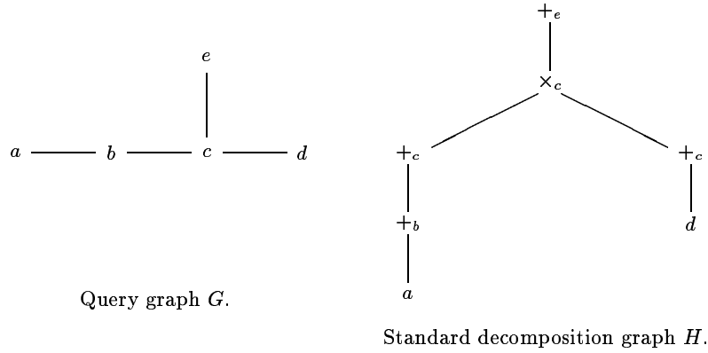
Fig. 5. Query graph and standard decomposition graph.
