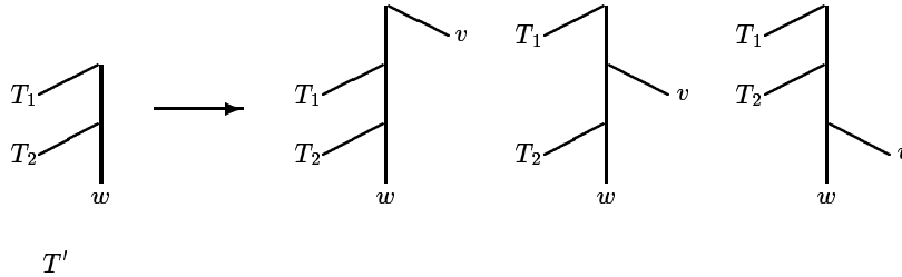
Fig. 3. Construction by leaf-insertion.
