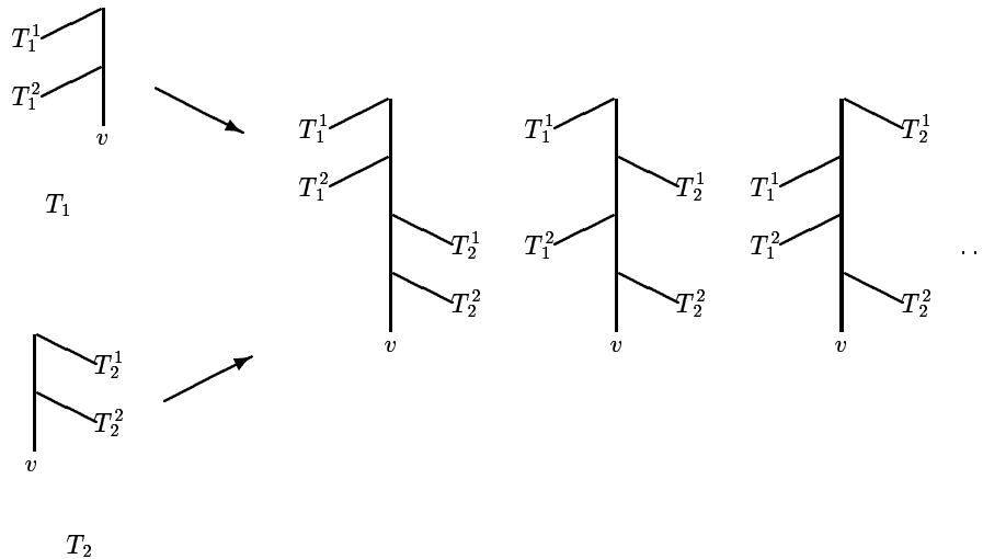
Fig. 4. Construction by tree-merging.
